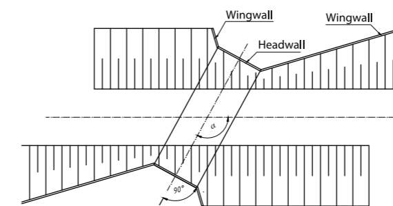
Fig. 5. Skewed structure
